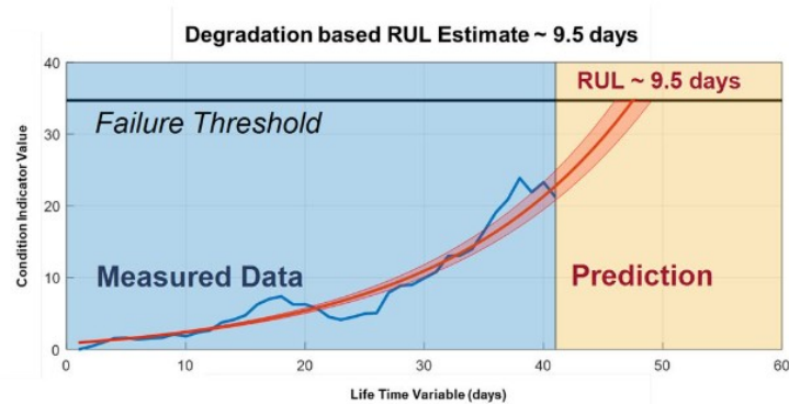
Figure 4-3 Degradation plot of a High-speed bearing in a wind turbine [19]
